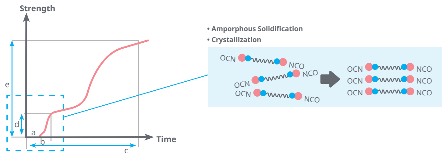
Figure 2. Physical crosslinking
