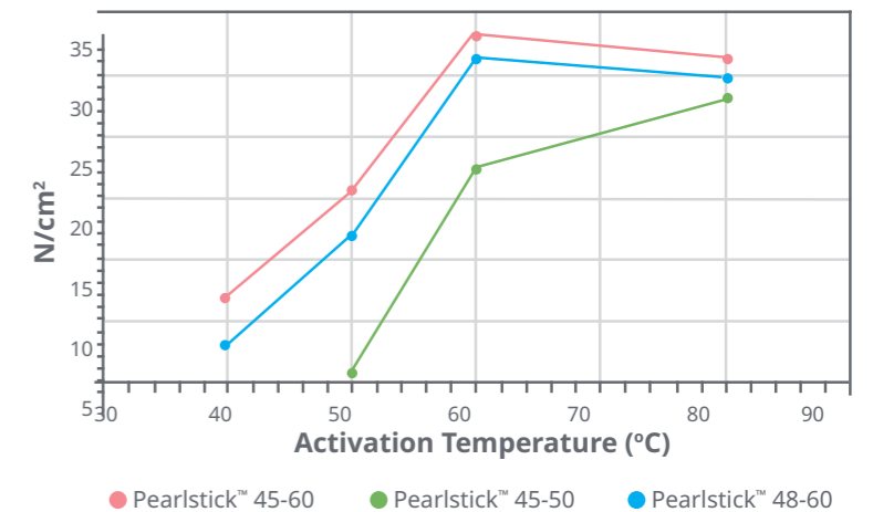
Hot-Tack 1 (PVC/Split leather) (Pressure: 2 kg/cm 2 , Contact time: 4 sec)
