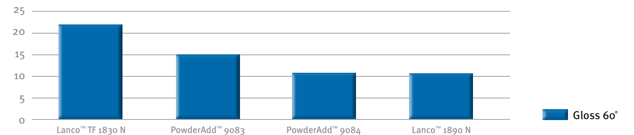
Matting Efficiency of Lanco™ & PowderAdd™ Texturing Agents
