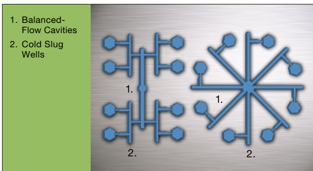
Figure 3: Runner Systems with Balanced-flow Cavity Layouts and Cold Slug Wells
