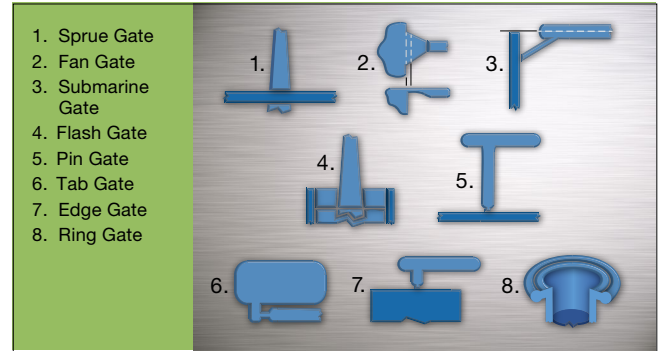
Figure 4: Gate Designs
