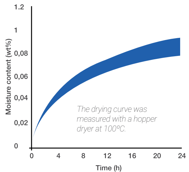
FIGURE 6: Drying and Moisture Absorption curves
