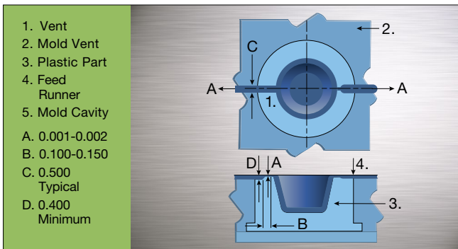
Figure 5: Mold Venting
