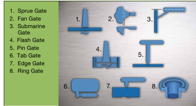
Figure 4: Gate Designs
